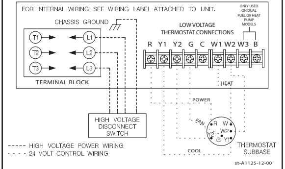
FIGURE 18 TYPICAL THERMOSTAT WIRING
