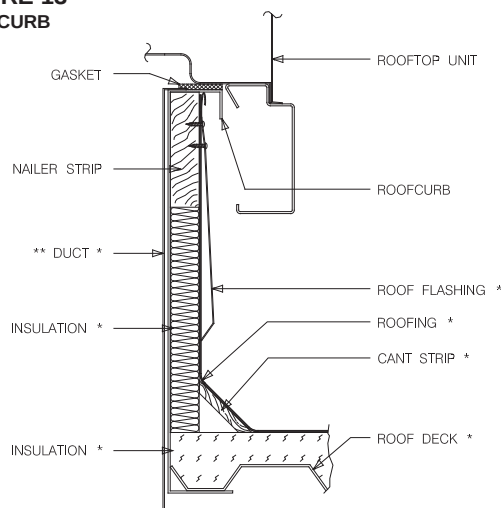
FIGURE 13 ROOFCURB
