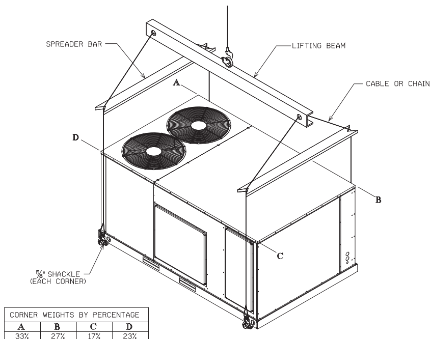
FIGURE 11 LIFTING DETAIL
